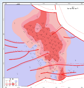
Sedimentary Characteristics
