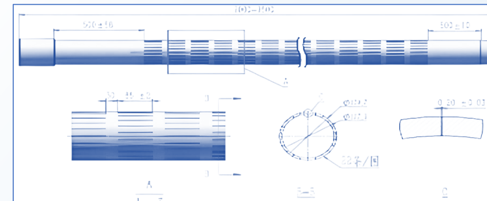
Plasma Slotted Screen Completion
